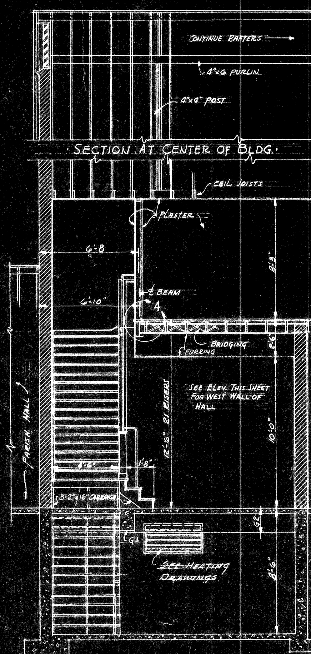
SECTION C-C SCALE 1/4" = 1'-0"
