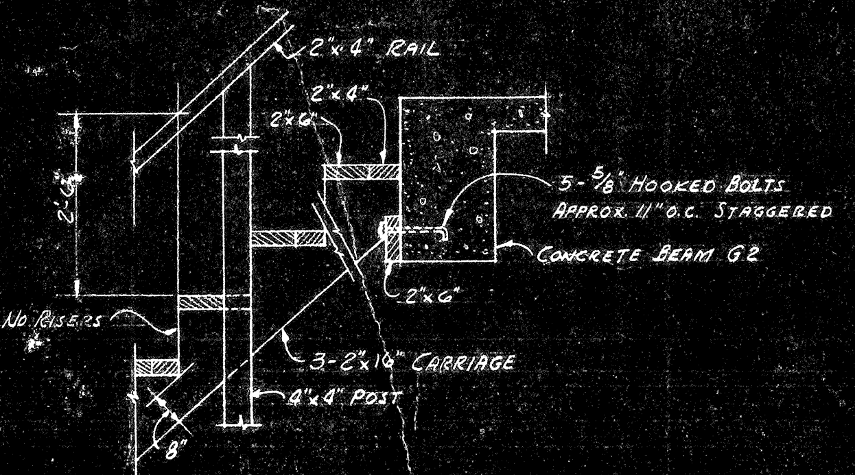
DETAIL OF BASEMENT STAIRWAY SCALE 3/4" = 1'-0"
