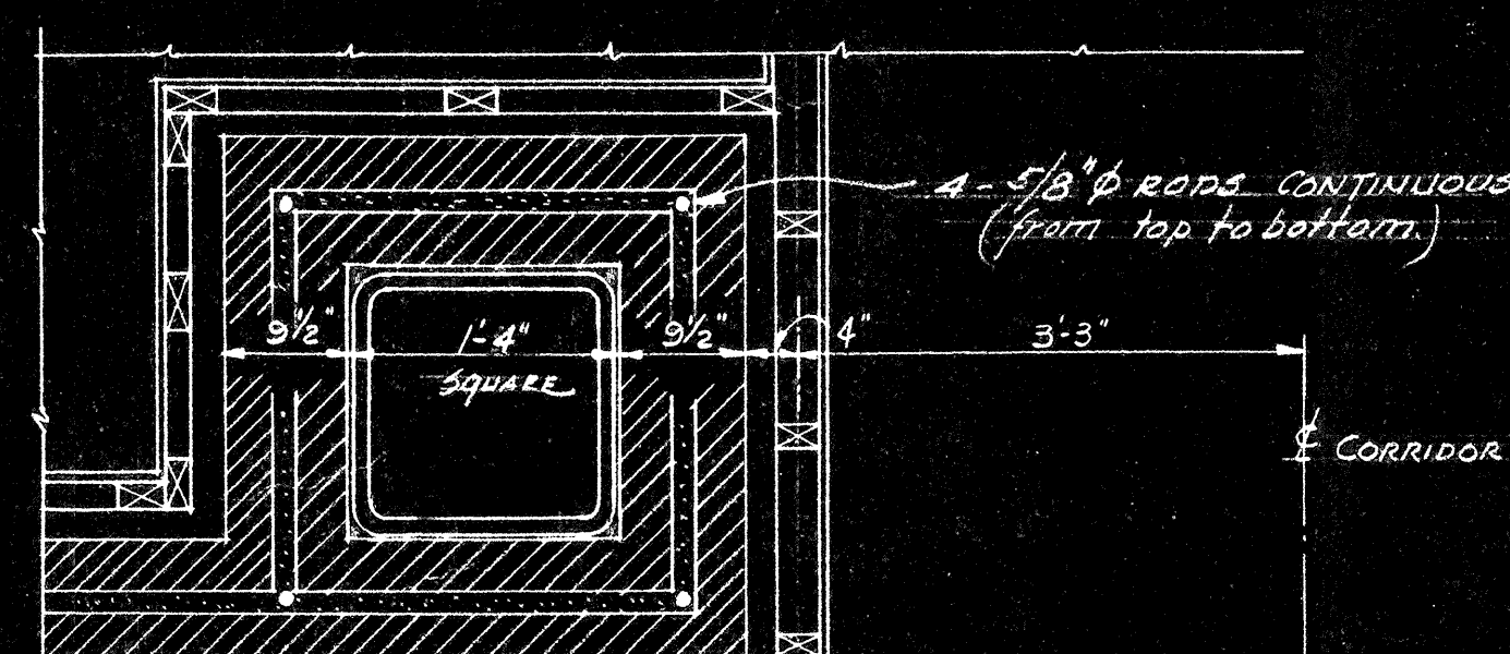
PLAN SECTION OF CHIMNEY
