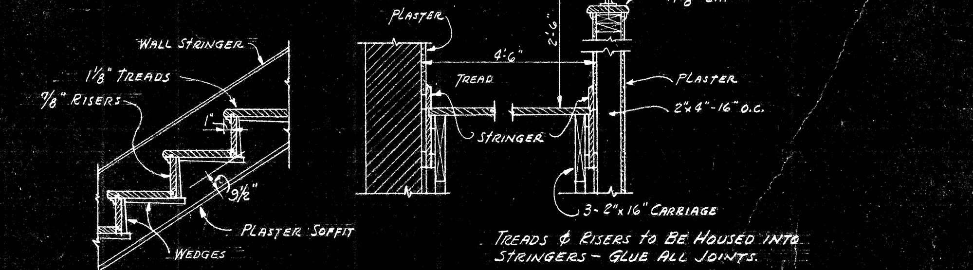
FIRST TO SECOND FL. STAIR DETAILS SCALE 3/4" = 1'-0"
