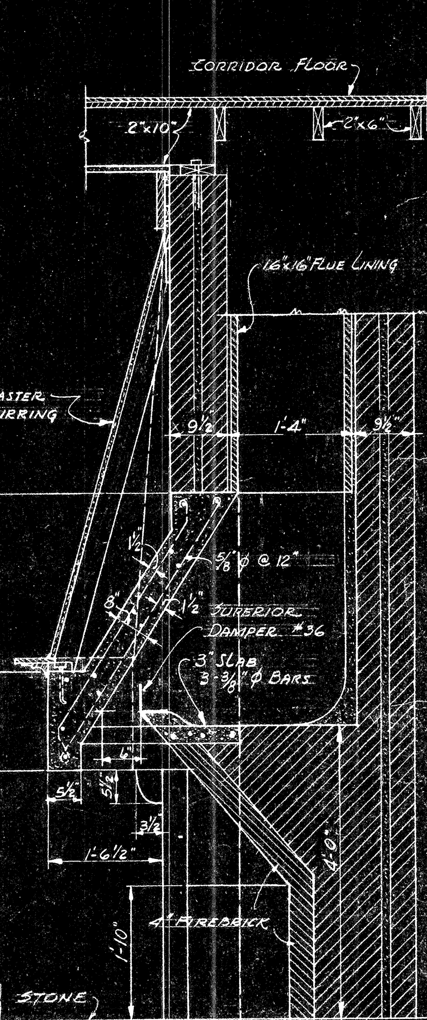
SECTION
