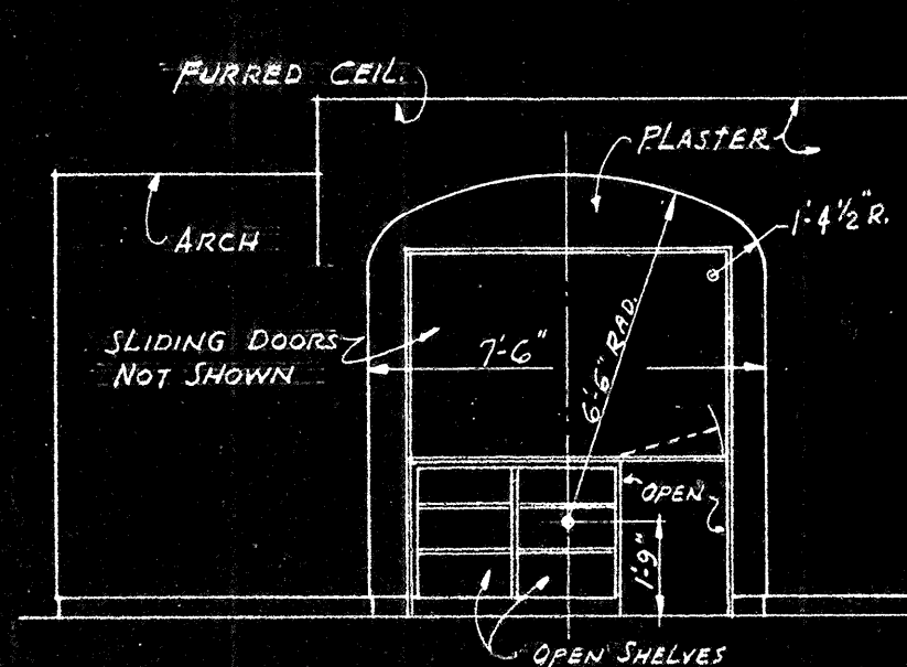
ELEVATION - WEST WALL OF HALL SCALE 1/4" = 1'-0"
