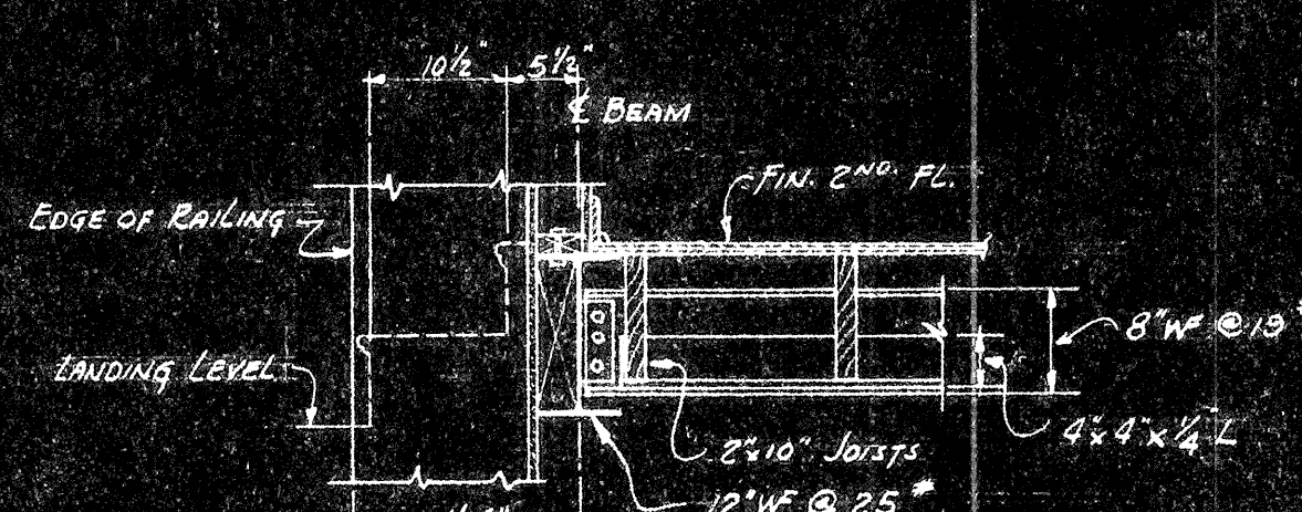
DETAIL 4 SCALE 3/4" = 1'-0"
